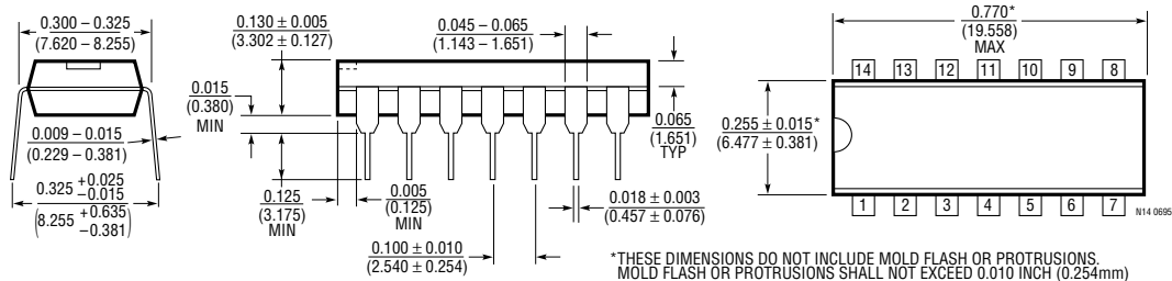
S Package 14-Lead Plastic SO
